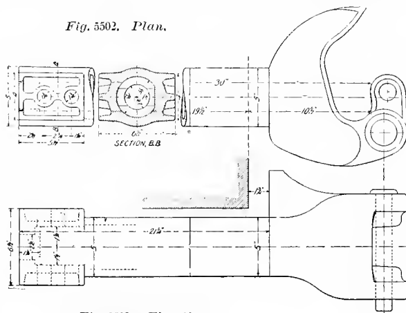
Fig. 5503. Elevation. MASTER CAR BUILDERS' STANDARD AUTOMATIC CAR-COUPLER. (Adopted in 1887. Further details adopted in 1889 and 1893.)
